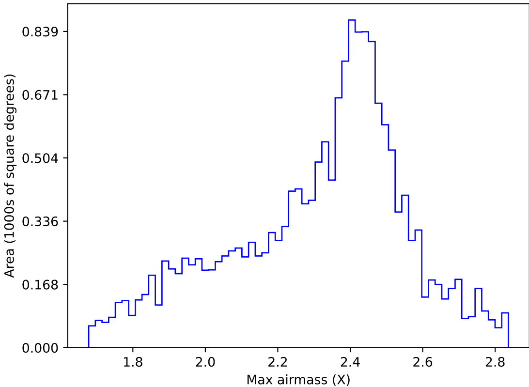
too_elab_r16_d3_giz_v3.4_10yrs WFD r band: Max airmass
