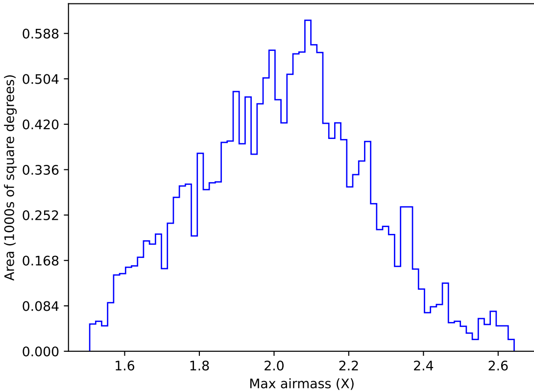
too_elab_r16_d3_giz_v3.4_10yrs WFD g band: Max airmass
