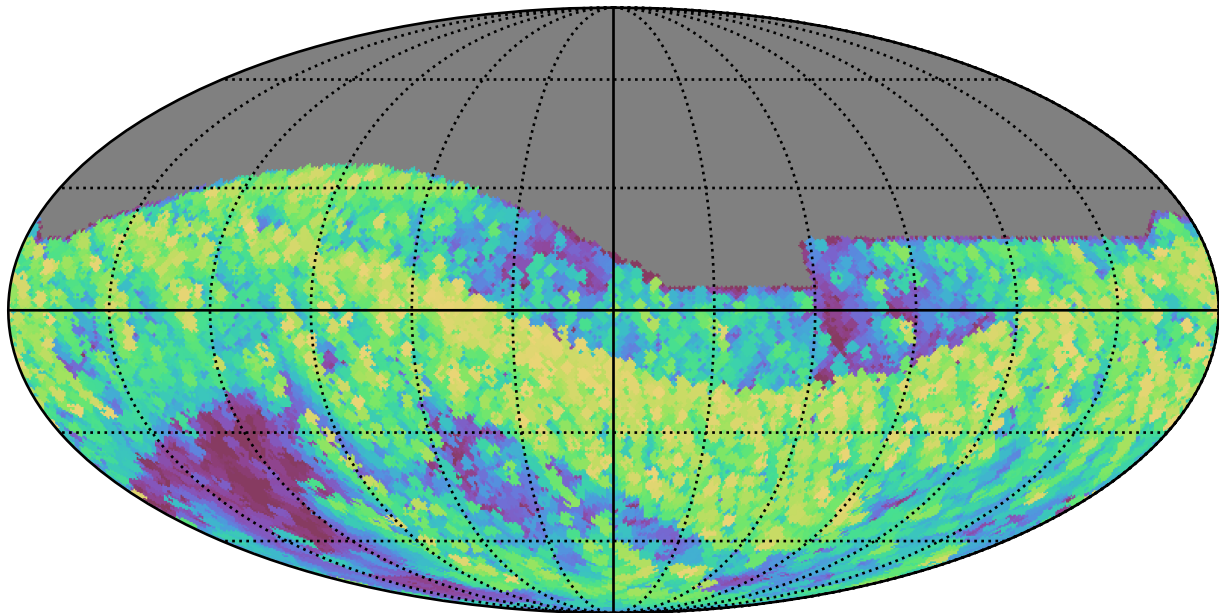
too_elab_r16_d3_giz_v3.4_10yrs All sky z band: Max airmass
