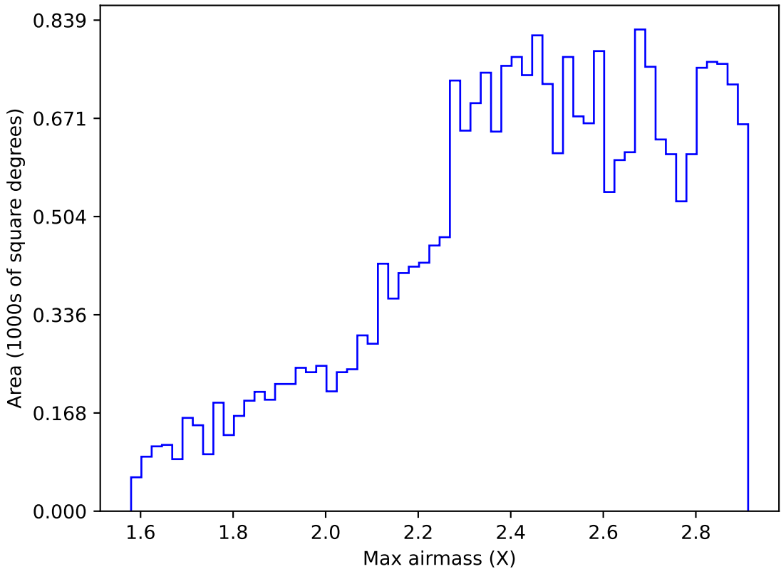
too_elab_r16_d3_giz_v3.4_10yrs All sky z band: Max airmass
