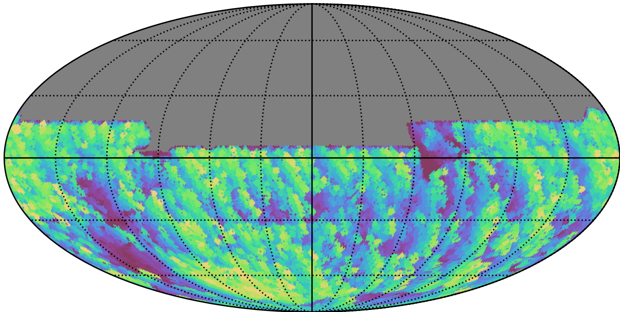
too_elab_r16_d3_giz_v3.4_10yrs All sky y band: Max airmass
