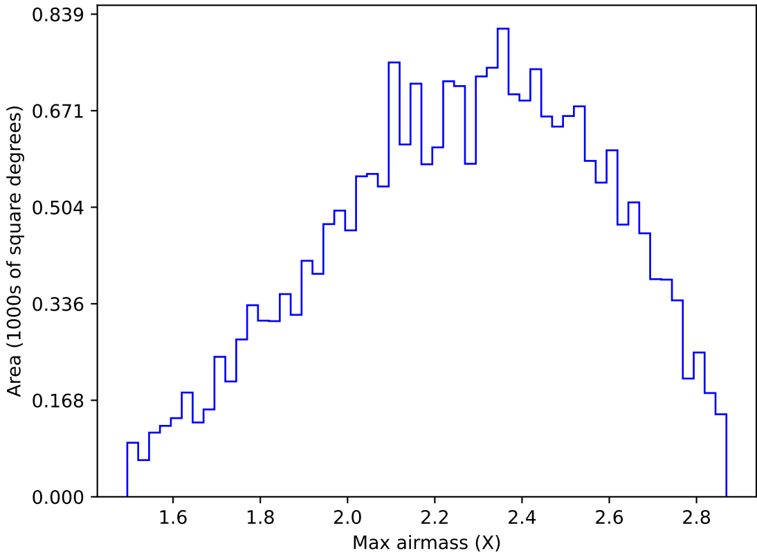
too_elab_r16_d3_giz_v3.4_10yrs All sky y band: Max airmass
