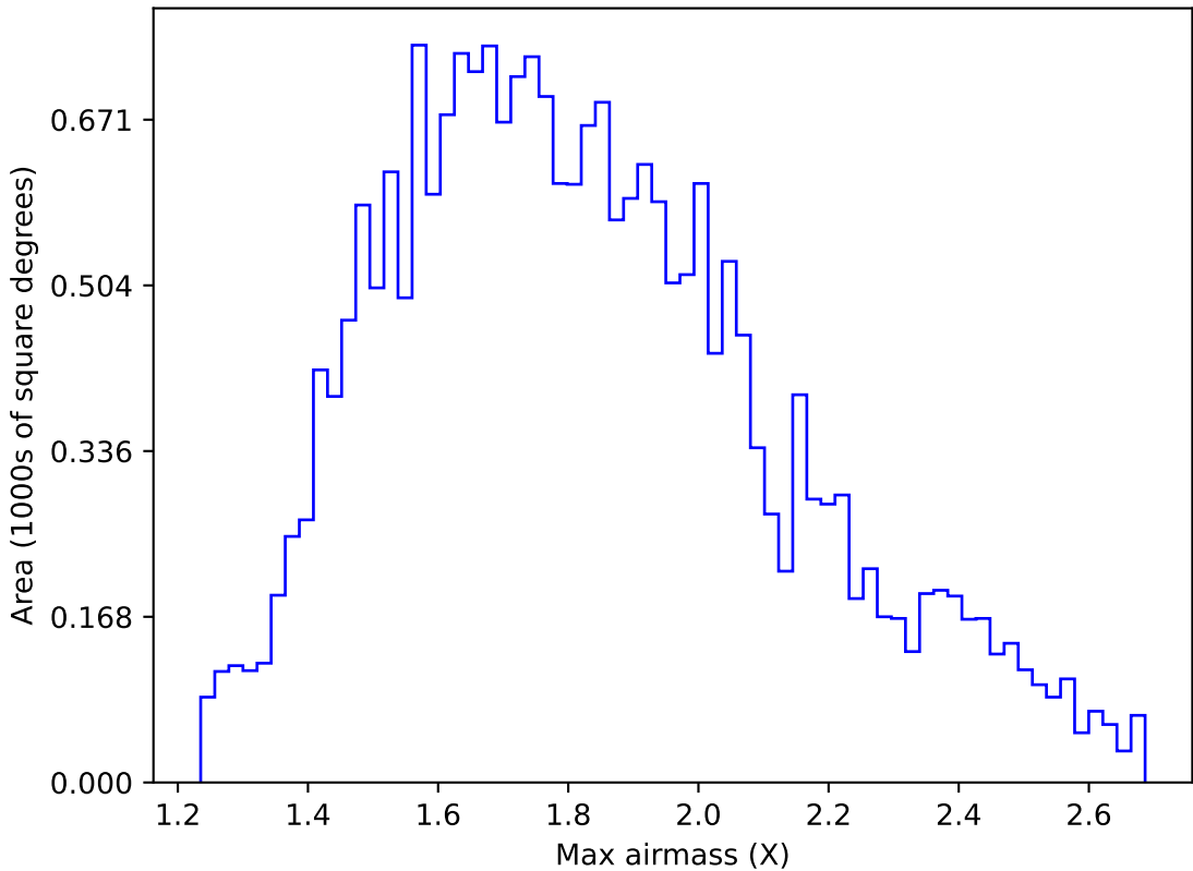
too_elab_r16_d3_giz_v3.4_10yrs All sky u band: Max airmass
