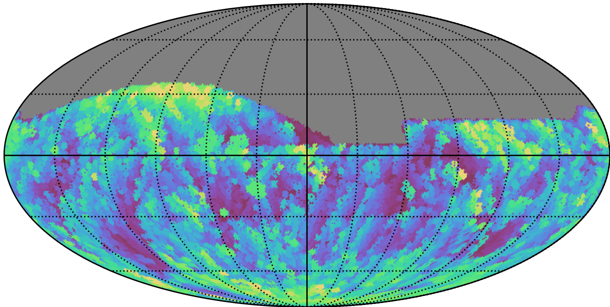
too_elab_r16_d3_giz_v3.4_10yrs All sky g band: Max airmass
