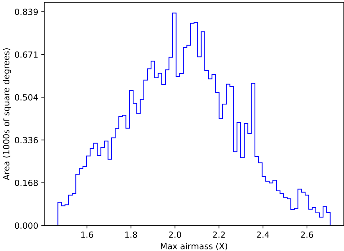
too_elab_r16_d3_giz_v3.4_10yrs All sky g band: Max airmass
