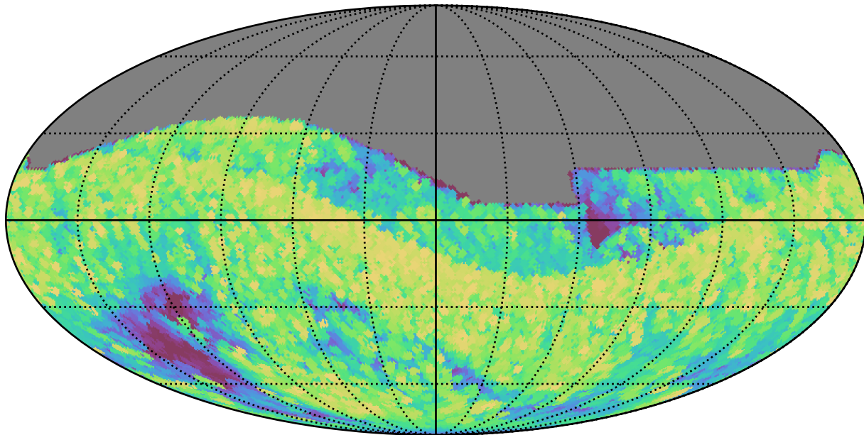
too_elab_r16_d3_giz_v3.4_10yrs All sky all bands: Max airmass
