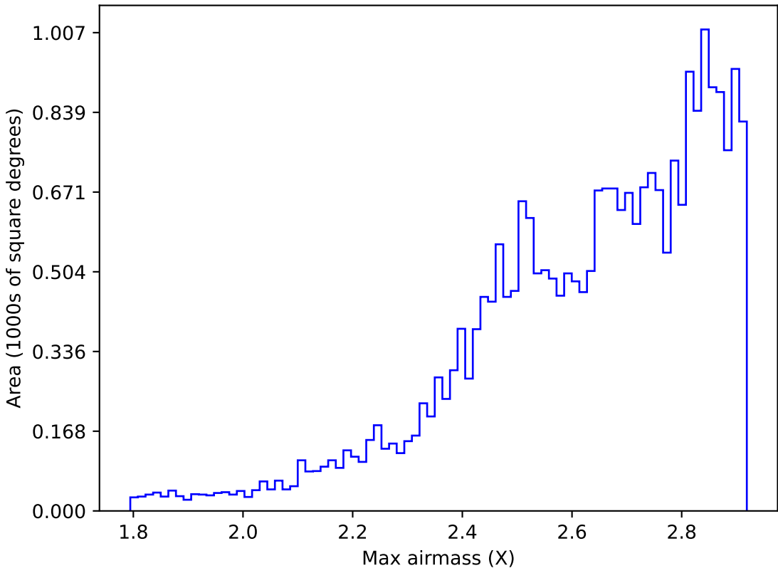
too_elab_r16_d3_giz_v3.4_10yrs All sky all bands: Max airmass
