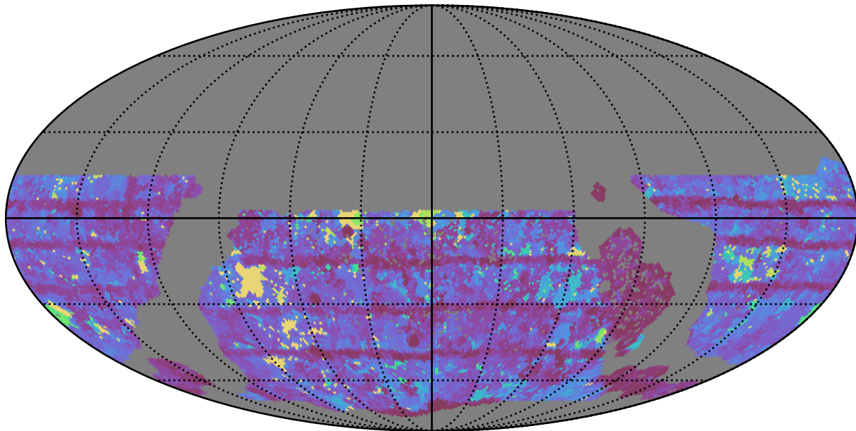
too_elab_r16_d3_giz_v3.4_10yrs WFD z band: Max Inter-Night Gap
