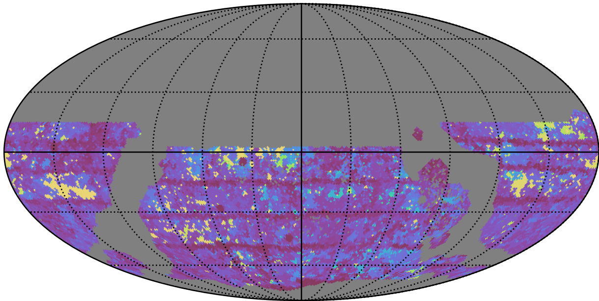
too_elab_r16_d3_giz_v3.4_10yrs WFD y band: Max Inter-Night Gap
