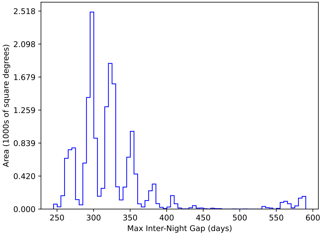
too_elab_r16_d3_giz_v3.4_10yrs WFD y band: Max Inter-Night Gap
