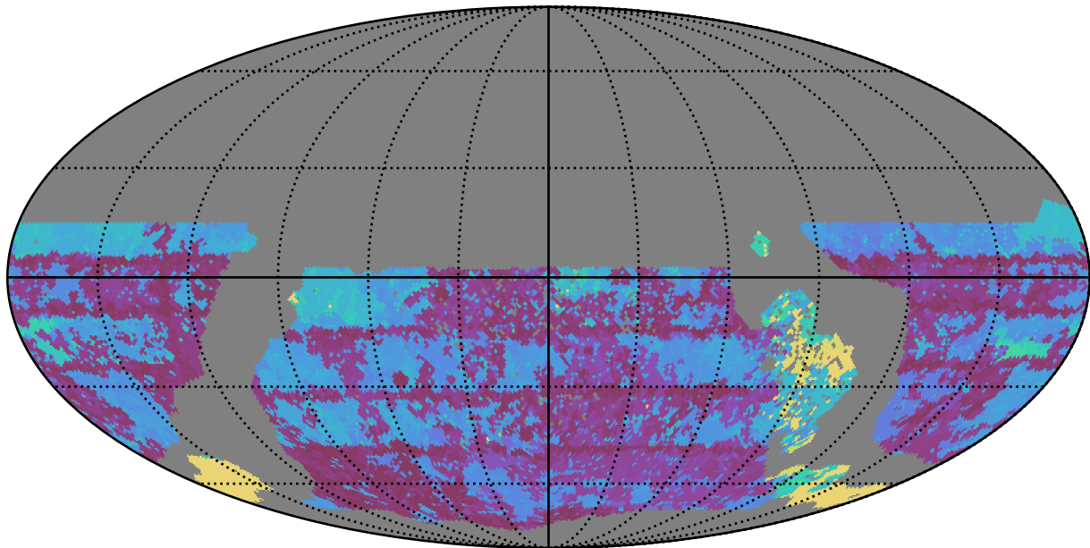
too_elab_r16_d3_giz_v3.4_10yrs WFD u band: Max Inter-Night Gap
