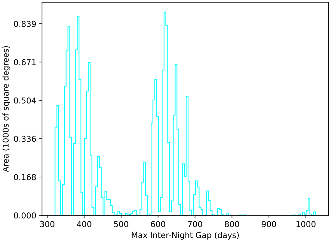
too_elab_r16_d3_giz_v3.4_10yrs WFD u band: Max Inter-Night Gap
