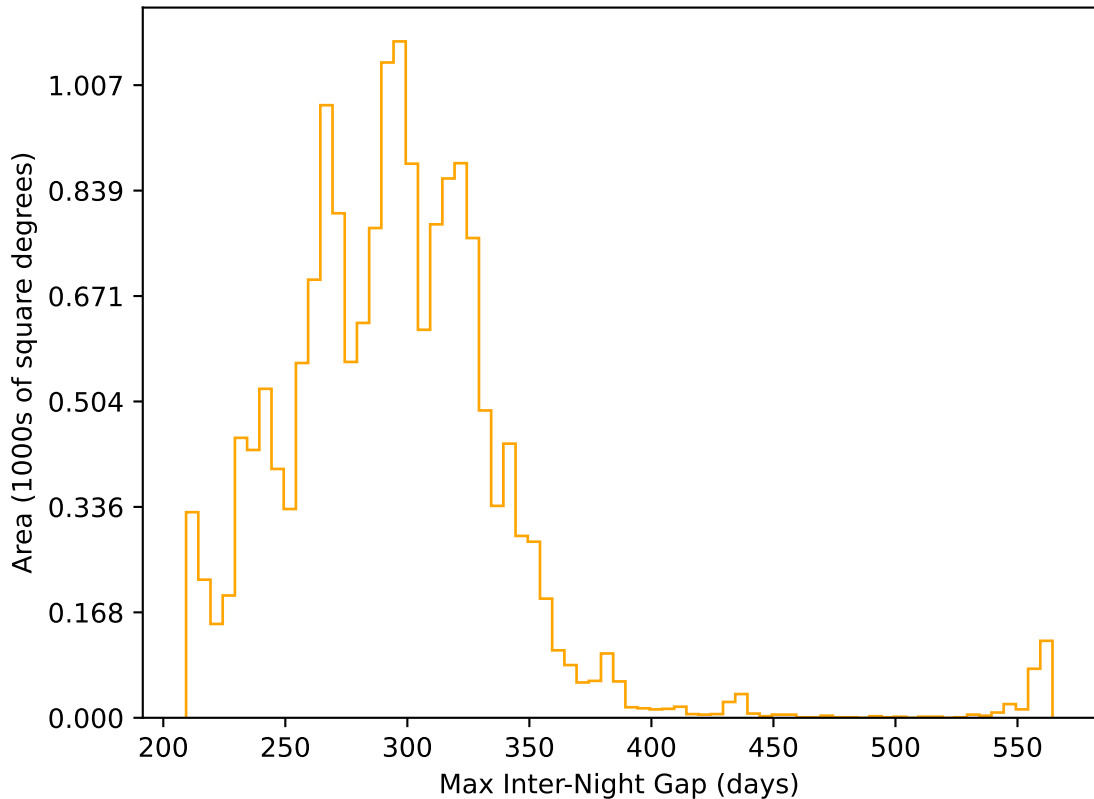
too_elab_r16_d3_giz_v3.4_10yrs WFD r band: Max Inter-Night Gap
