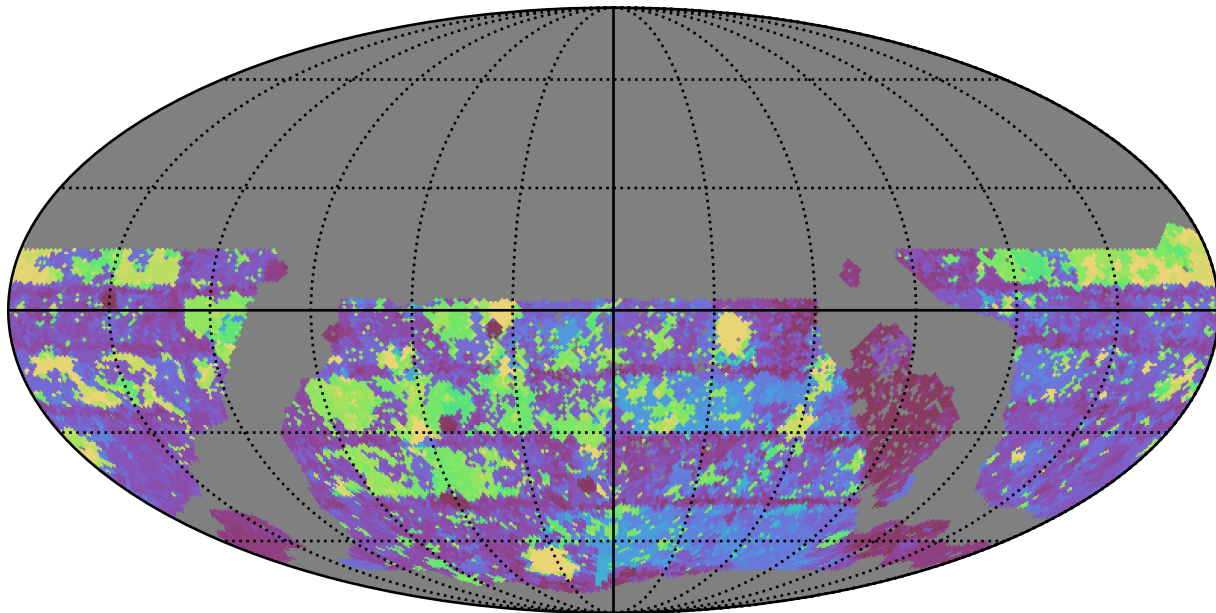
too_elab_r16_d3_giz_v3.4_10yrs WFD g band: Max Inter-Night Gap
