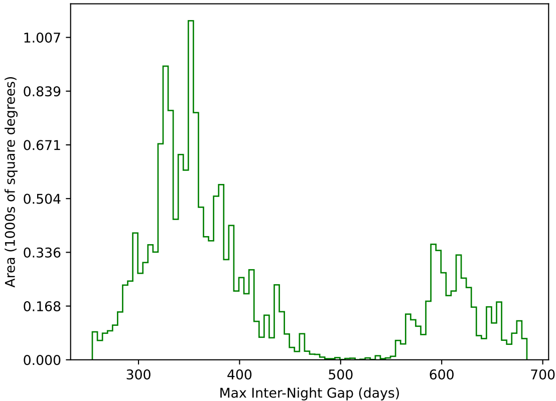
too_elab_r16_d3_giz_v3.4_10yrs WFD g band: Max Inter-Night Gap
