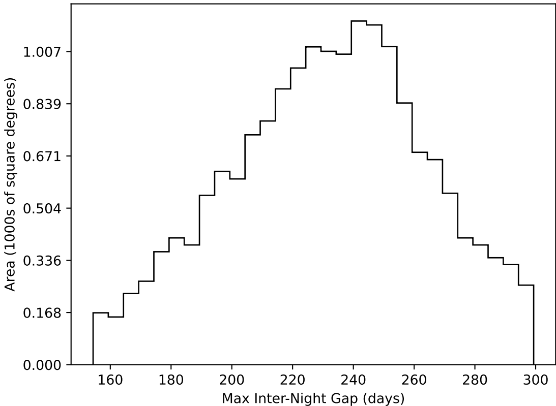
too_elab_r16_d3_giz_v3.4_10yrs WFD all bands: Max Inter-Night Gap
