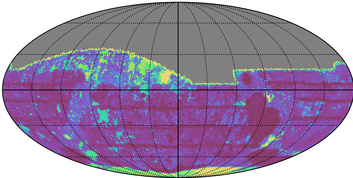
too_elab_r16_d3_giz_v3.4_10yrs All sky z band: Max Inter-Night Gap
