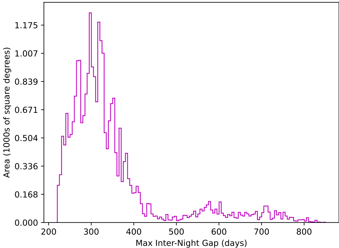
too_elab_r16_d3_giz_v3.4_10yrs All sky z band: Max Inter-Night Gap
