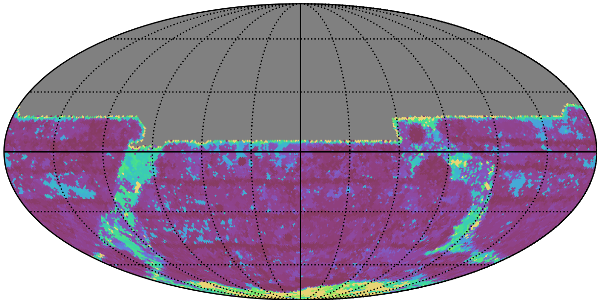
too_elab_r16_d3_giz_v3.4_10yrs All sky y band: Max Inter-Night Gap
