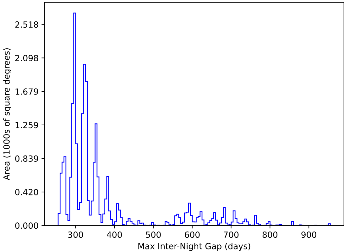
too_elab_r16_d3_giz_v3.4_10yrs All sky y band: Max Inter-Night Gap
