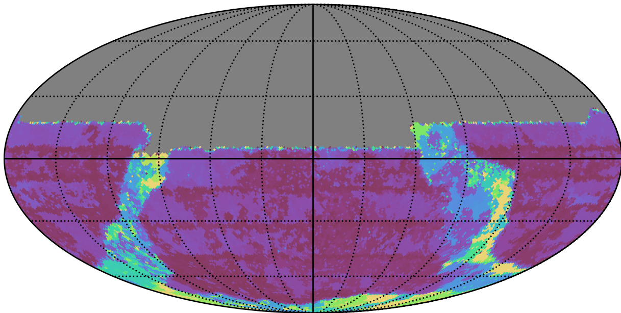
too_elab_r16_d3_giz_v3.4_10yrs All sky u band: Max Inter-Night Gap
