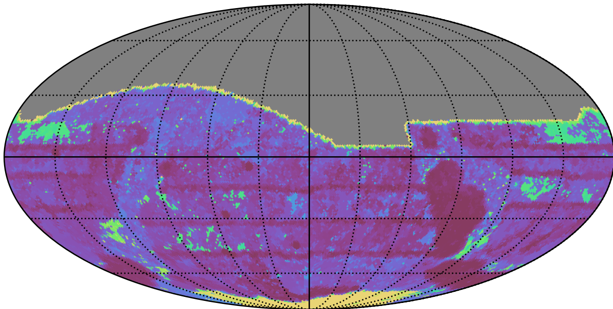
too_elab_r16_d3_giz_v3.4_10yrs All sky r band: Max Inter-Night Gap
