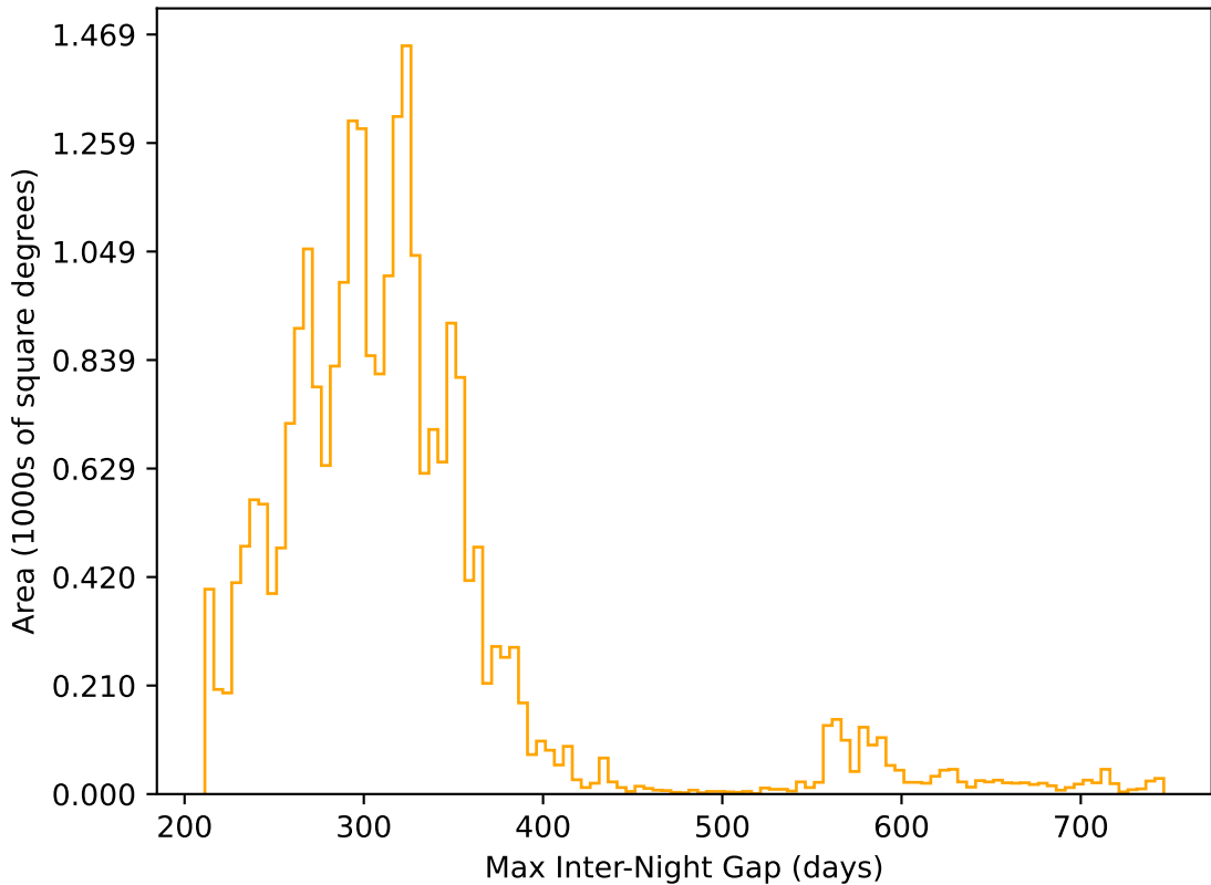
too_elab_r16_d3_giz_v3.4_10yrs All sky r band: Max Inter-Night Gap
