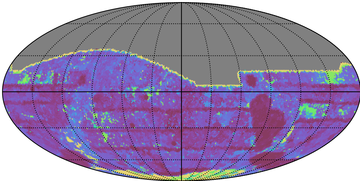
too_elab_r16_d3_giz_v3.4_10yrs All sky i band: Max Inter-Night Gap
