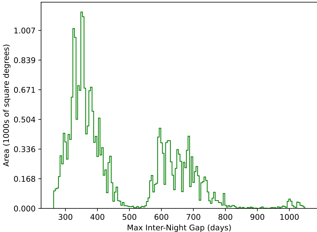
too_elab_r16_d3_giz_v3.4_10yrs All sky g band: Max Inter-Night Gap
