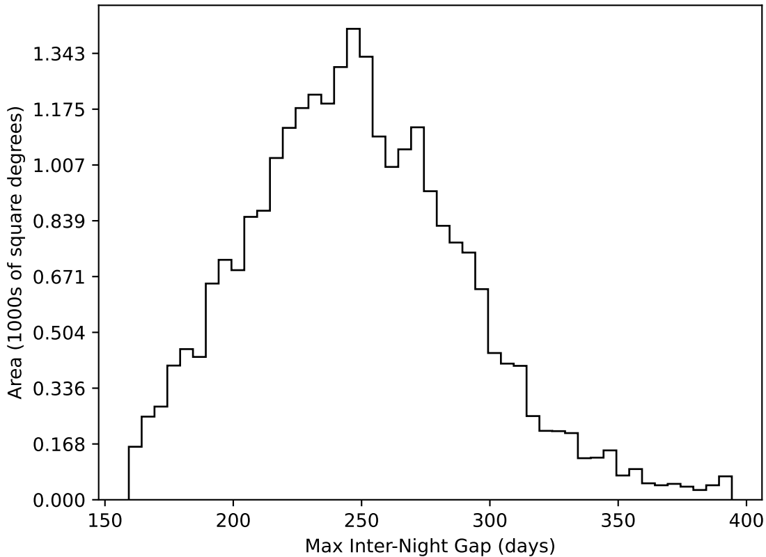
too_elab_r16_d3_giz_v3.4_10yrs All sky all bands: Max Inter-Night Gap
