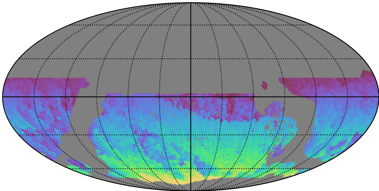
too_elab_r16_d3_giz_v3.4_10yrs WFD z band: Max HA
