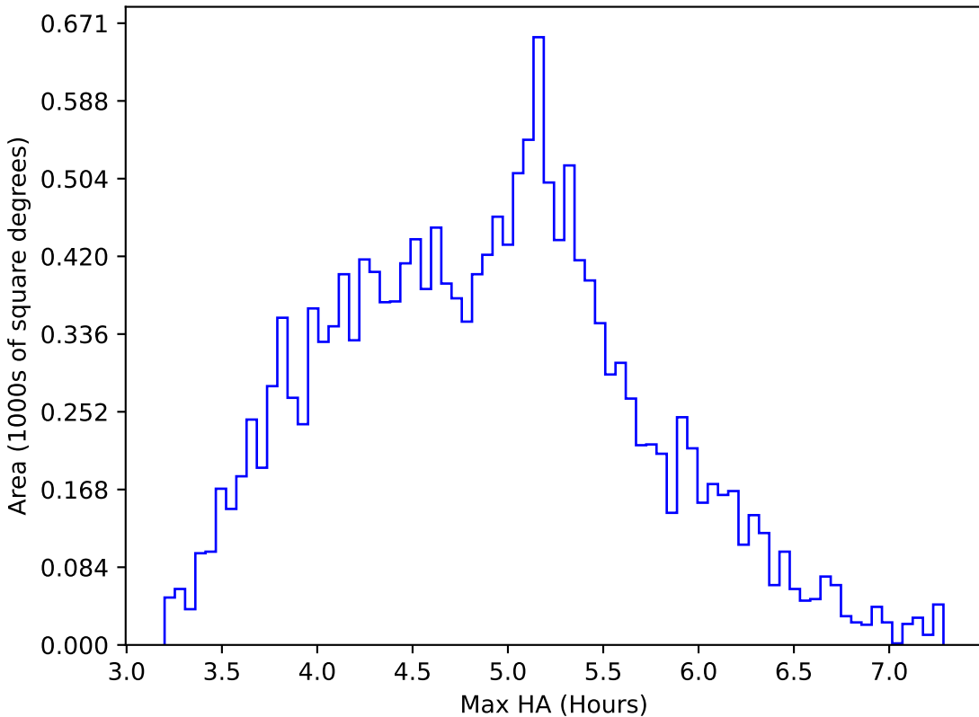
too_elab_r16_d3_giz_v3.4_10yrs WFD z band: Max HA
