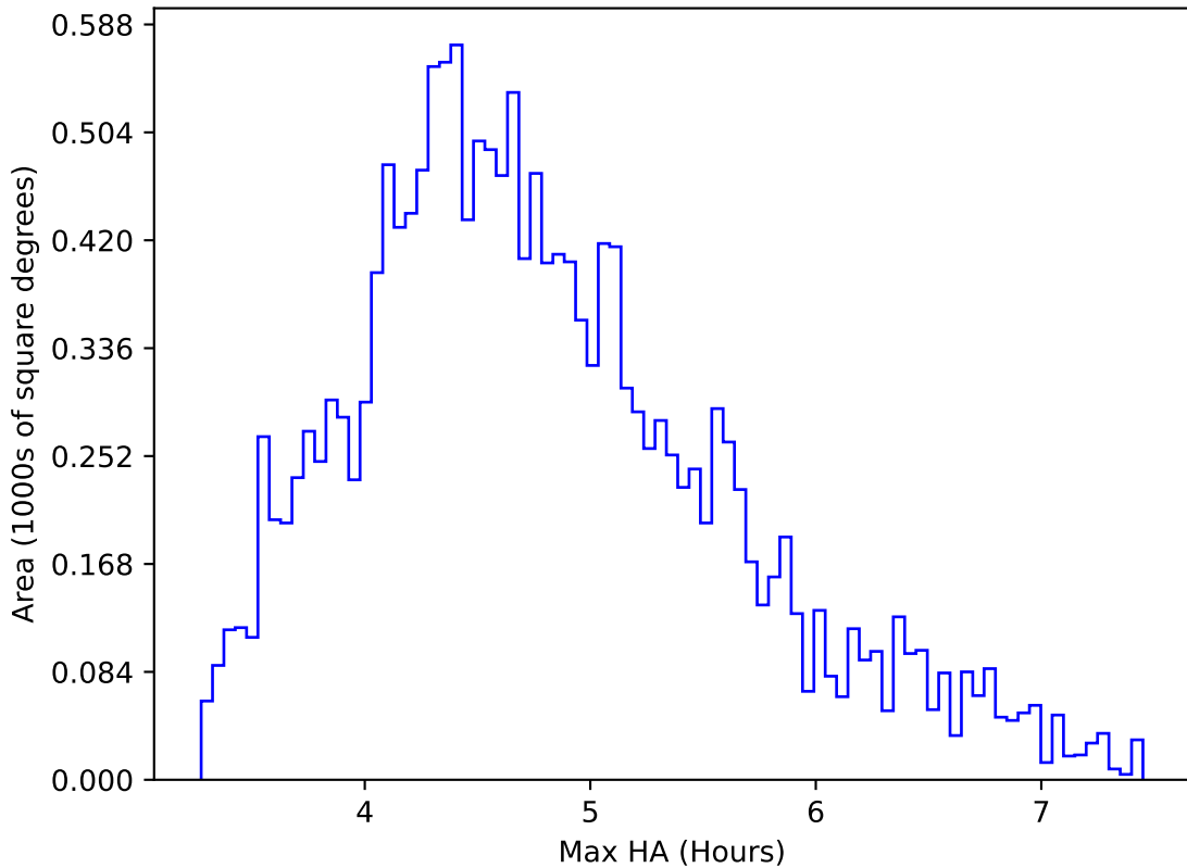
too_elab_r16_d3_giz_v3.4_10yrs WFD y band: Max HA
