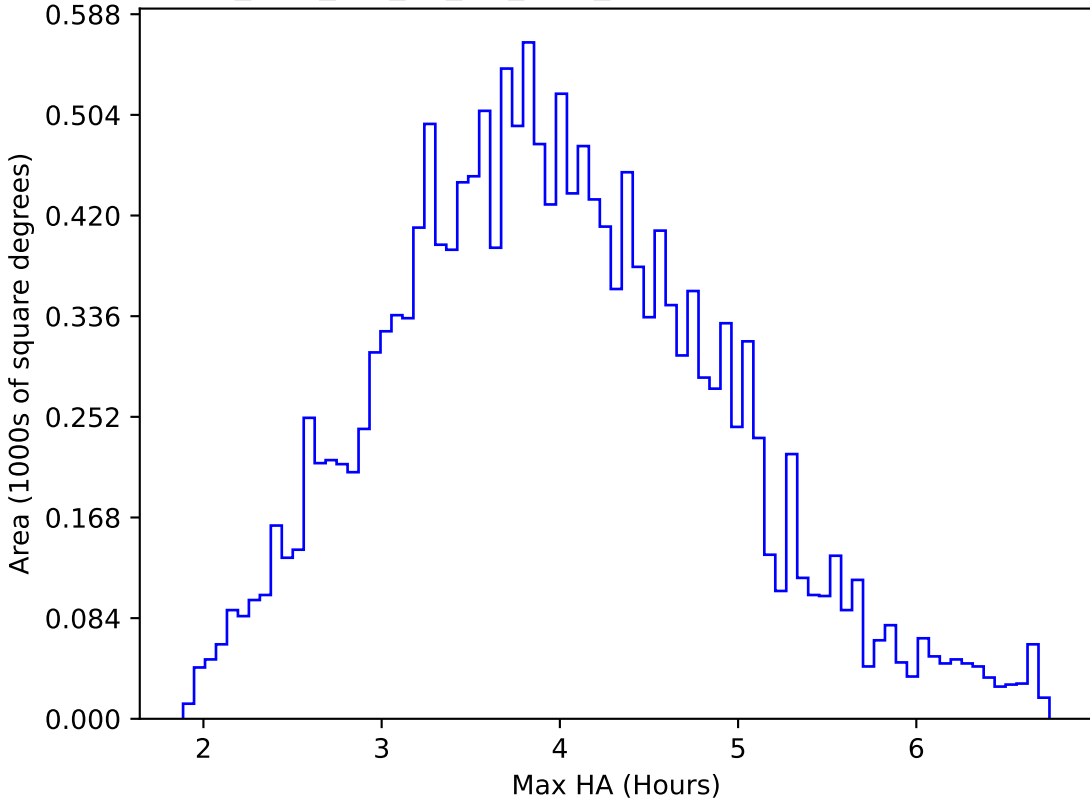
too_elab_r16_d3_giz_v3.4_10yrs WFD u band: Max HA
