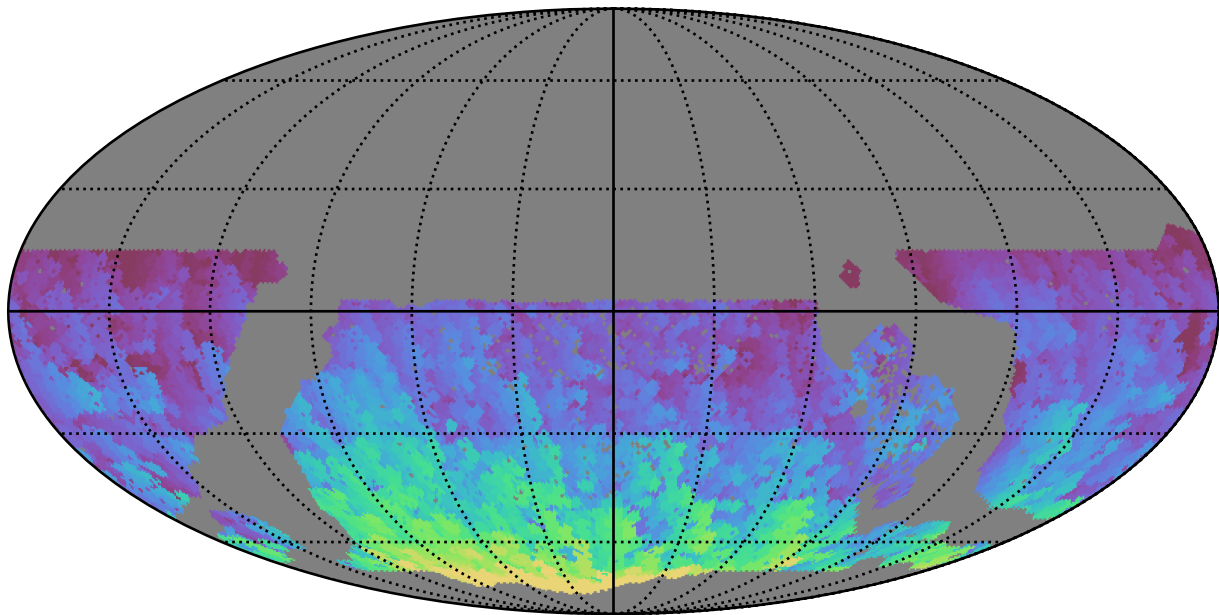
too_elab_r16_d3_giz_v3.4_10yrs WFD r band: Max HA
