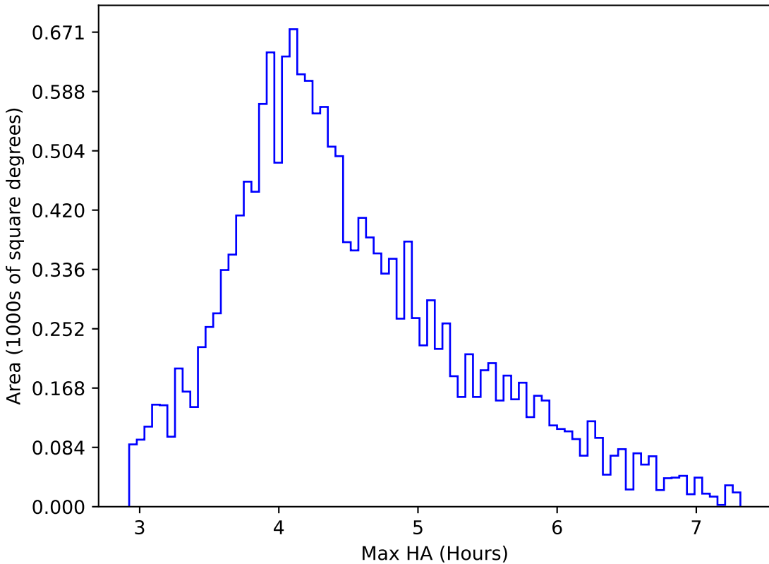
too_elab_r16_d3_giz_v3.4_10yrs WFD r band: Max HA
