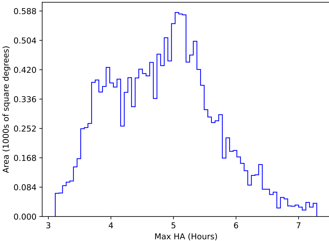
too_elab_r16_d3_giz_v3.4_10yrs WFD i band: Max HA
