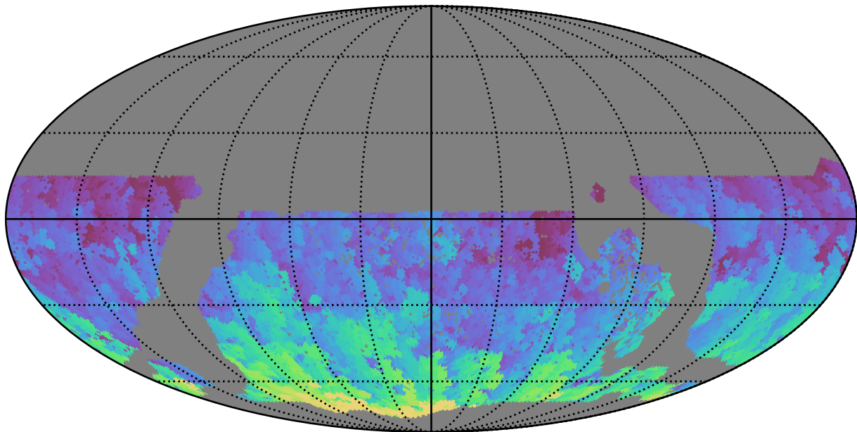
too_elab_r16_d3_giz_v3.4_10yrs WFD g band: Max HA
