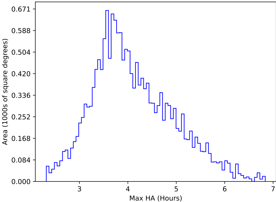
too_elab_r16_d3_giz_v3.4_10yrs WFD g band: Max HA
