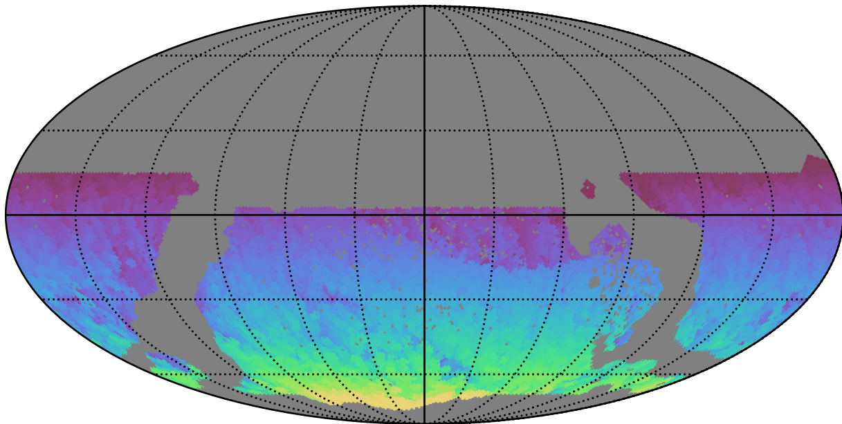
too_elab_r16_d3_giz_v3.4_10yrs WFD all bands: Max HA
