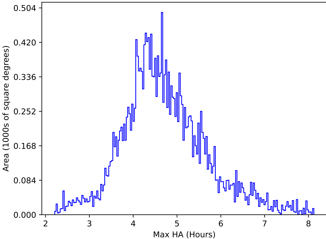
too_elab_r16_d3_giz_v3.4_10yrs All sky y band: Max HA
