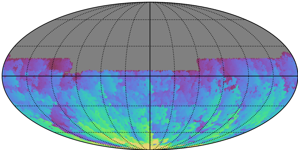
too_elab_r16_d3_giz_v3.4_10yrs All sky u band: Max HA
