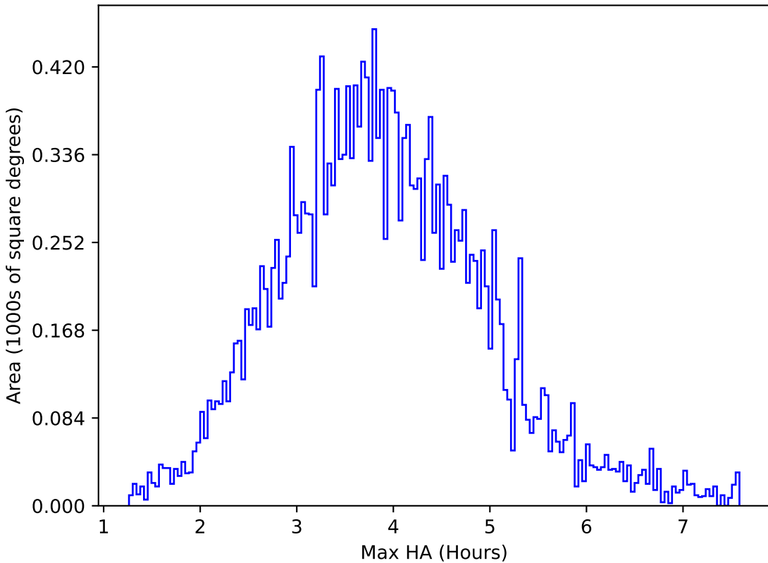
too_elab_r16_d3_giz_v3.4_10yrs All sky u band: Max HA
