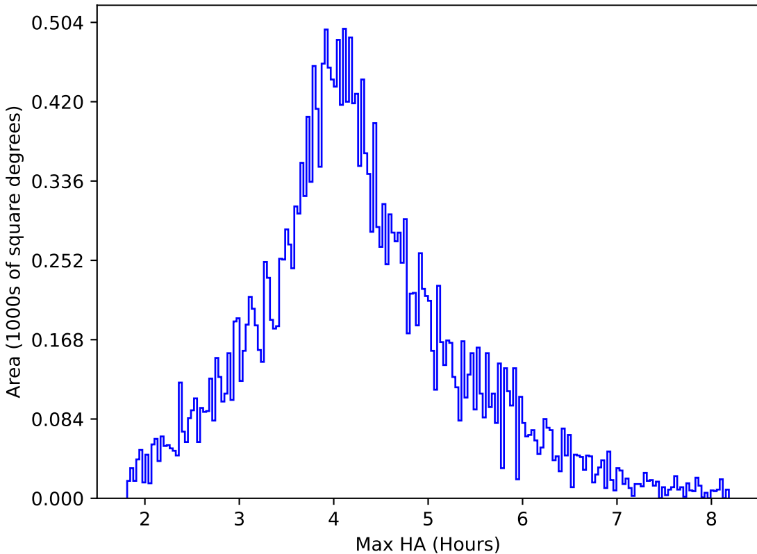
too_elab_r16_d3_giz_v3.4_10yrs All sky r band: Max HA
