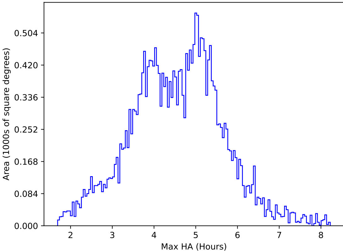
too_elab_r16_d3_giz_v3.4_10yrs All sky i band: Max HA
