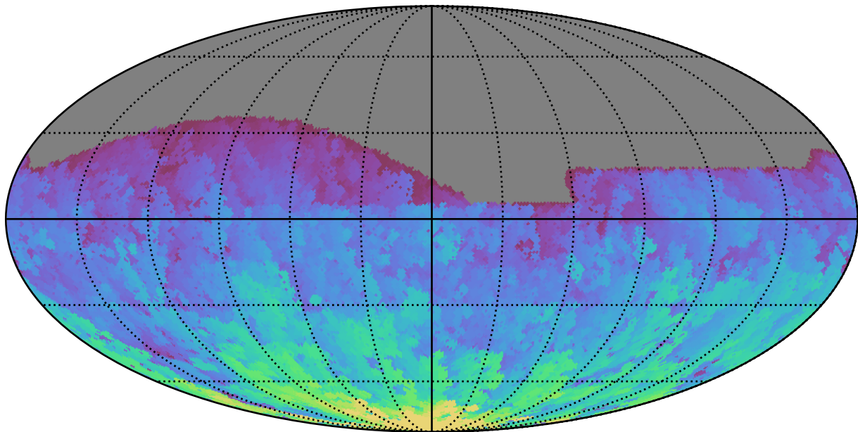
too_elab_r16_d3_giz_v3.4_10yrs All sky g band: Max HA
