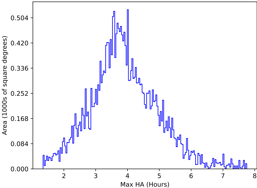
too_elab_r16_d3_giz_v3.4_10yrs All sky g band: Max HA
