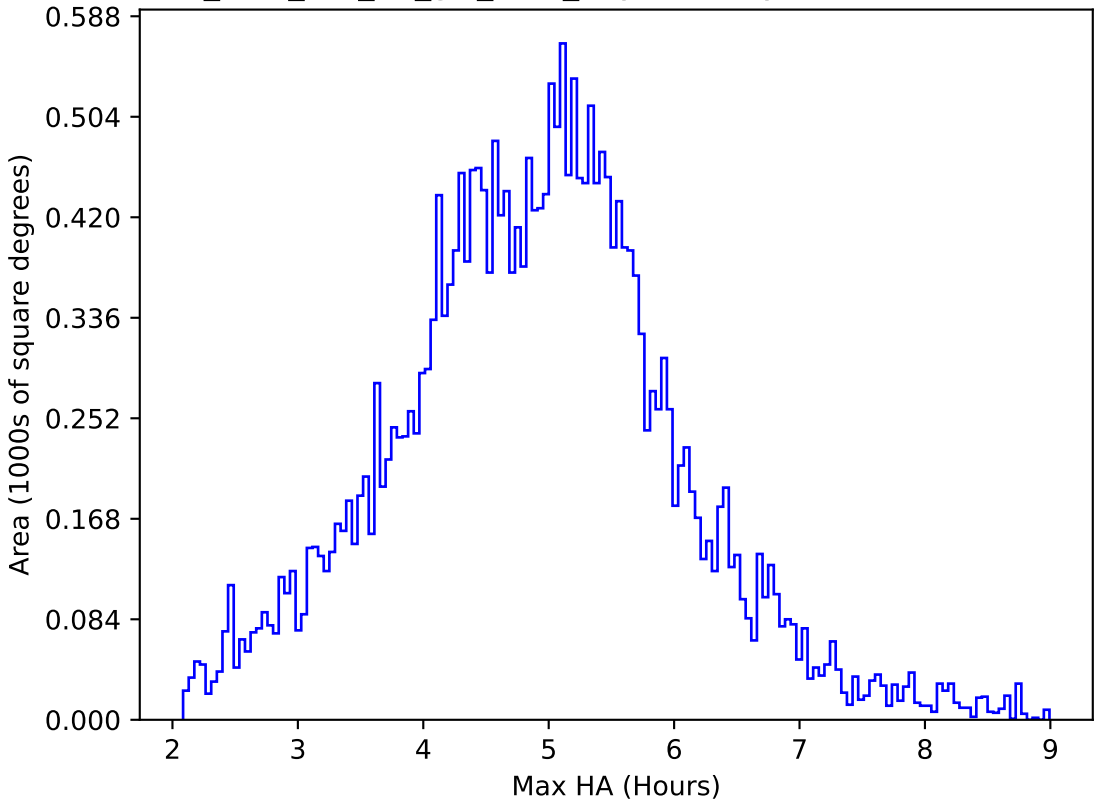
too_elab_r16_d3_giz_v3.4_10yrs All sky all bands: Max HA
