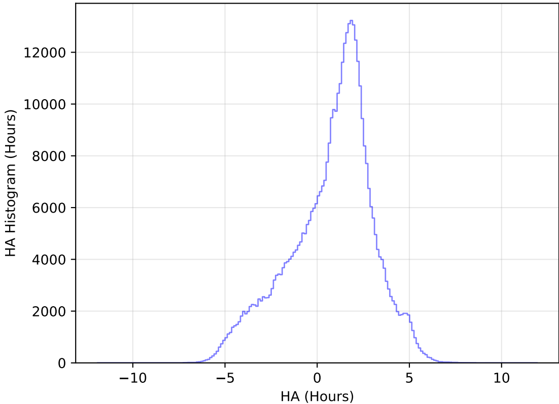
too_elab_r16_d3_giz_v3.4_10yrs WFD z band: HA Histogram
