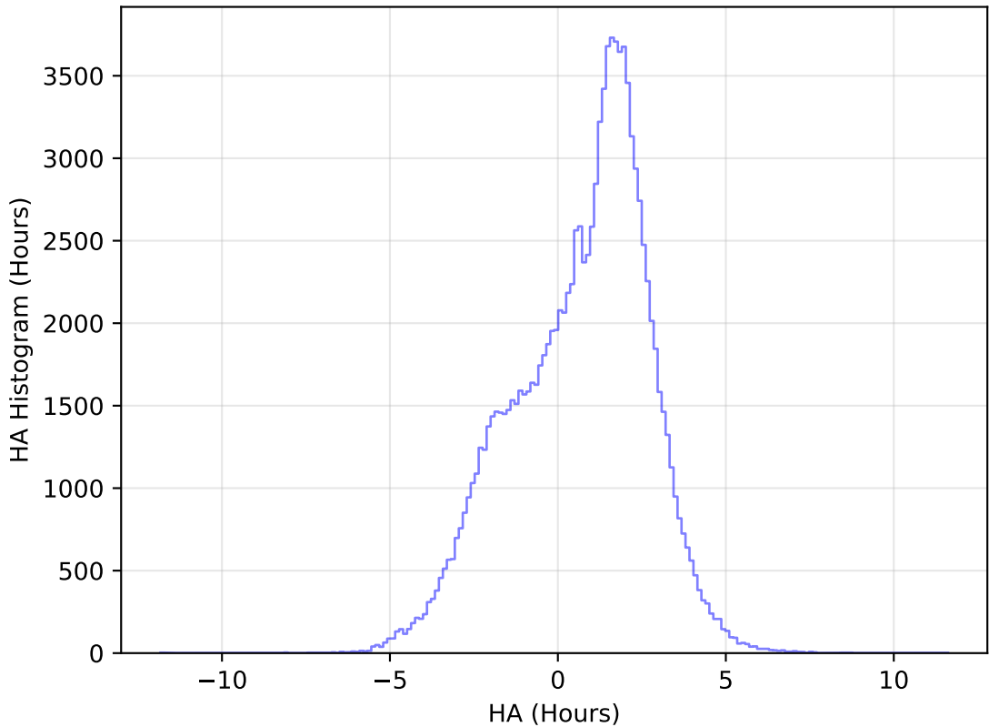
too_elab_r16_d3_giz_v3.4_10yrs WFD u band: HA Histogram
